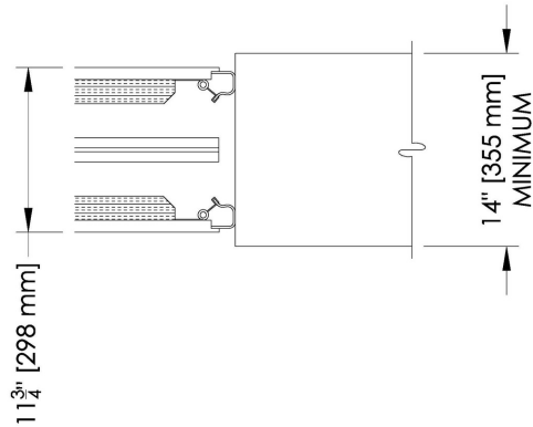
SQUARE/RECTANGULAR COLUMN DETAILS
