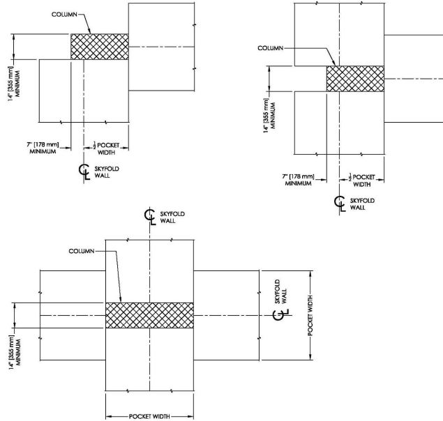
MULTIPLE SKYFOLD WALLS COLUMN DETAILS
