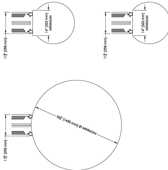
ROUND COLUMN DETAILS
